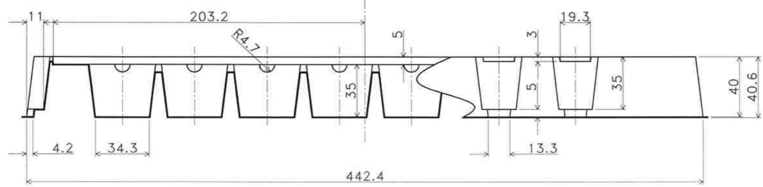
SECTION "X-X"
