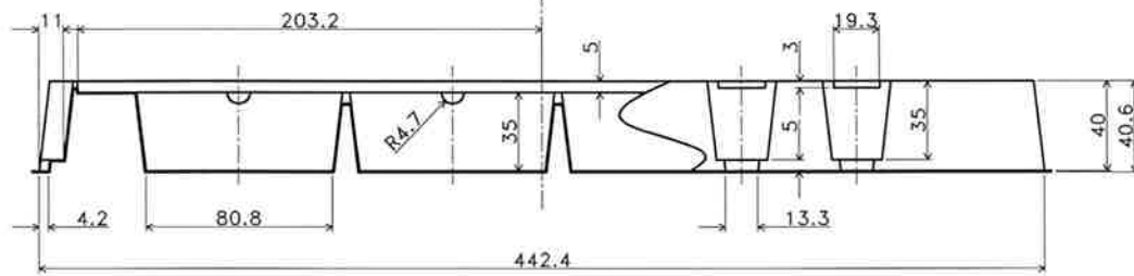
SECTION "X-X"
