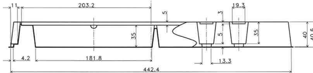
SECTION "X-X"
