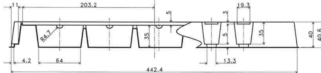
SECTION "X-X"
