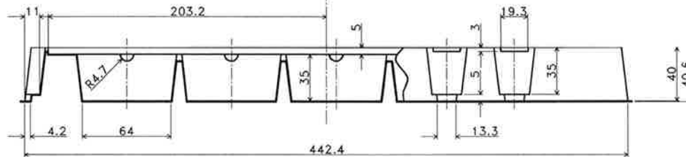
SECTION "X-X"
