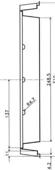
SECTION "Y-Y"
