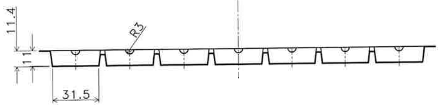
SECTION "X-X"
